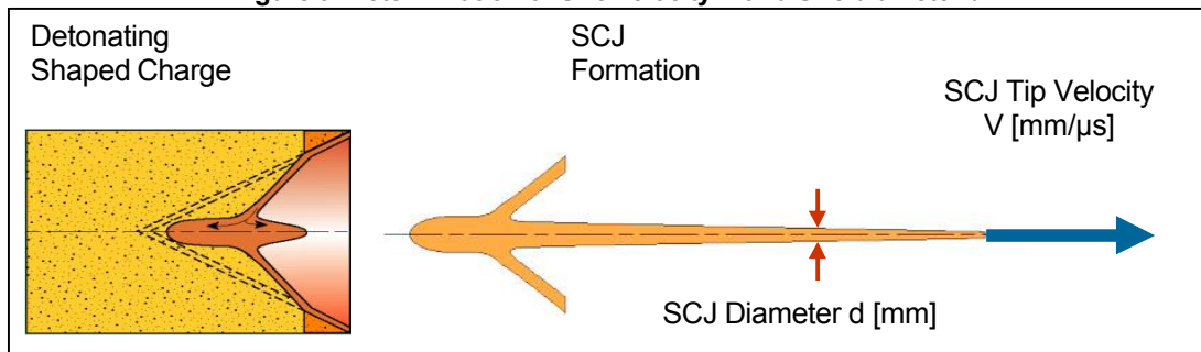
Figure 3: Determination of SCJ velocity V and SCJ diameter d
